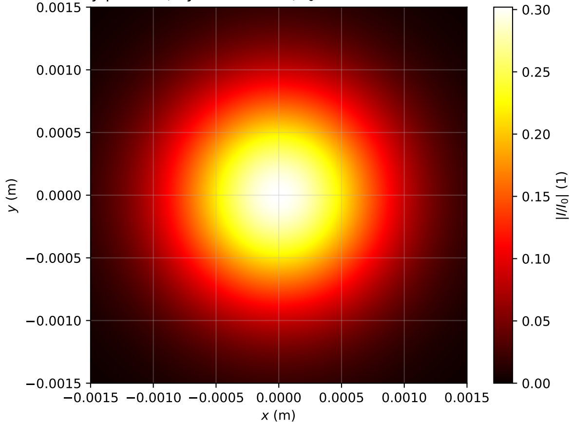
Intensity profile I(x, y, z = 3.821m)/I_0 , P_{in}=0.3P_{cr} , artificial time
